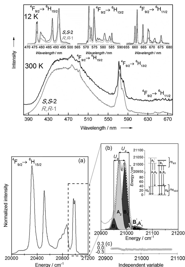
Figure 4. Top: Emission spectrum of R,R -1 and S,S -2 acquired at room temperature and at 12 K ( \lambda_{\text{exc}} = 365 nm). Bottom: a) Magnification of the ^4\text{F}_{9/2} \rightarrow ^6\text{H}_{15/2} transition for S,S -2 at 12 K. b) Multi-Gaussian functions fit (○) and the components from the first ^4\text{F}_{9/2} Stark sublevels to the ^6\text{H}_{15/2} multiplet in the range 20900–21100 \text{cm}^{-1} . A 1 ' and B 1 ' denote hot bands arising from transitions from the first ^4\text{F}_{9/2} Stark sublevel to the ground level of the ^6\text{H}_{15/2} multiplet. c) Residual plot ( R^2 \approx 0.98 ) for a judgment of the fit quality.
